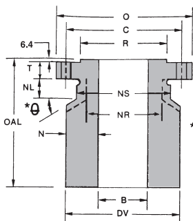
Conneessioni rinforzate Reinforced connection "V 2 "
