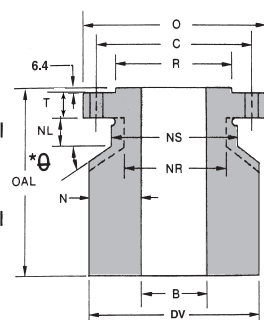
Conneessioni rinforzate Reinforced connection "V 3 "
